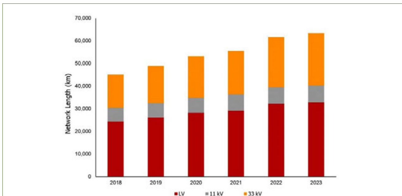
Figure 65: The electricity distribution network across the Uganda.
